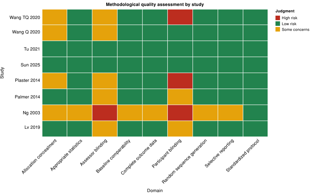
FIGURE 2. Methodological quality assessment by individual study (traffic-light plot).
