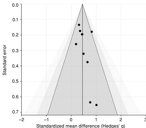
FIGURE 9. Contour-enhanced funnel plot for the continuous-outcome model.
