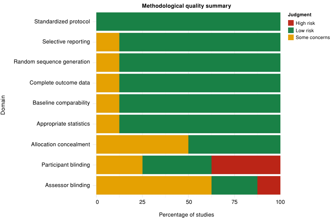
FIGURE 3. Summary of methodological quality across all included studies.
