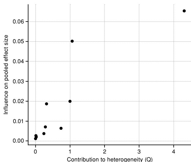
FIGURE 8. Baujat plot identifying influential continuous comparisons.
