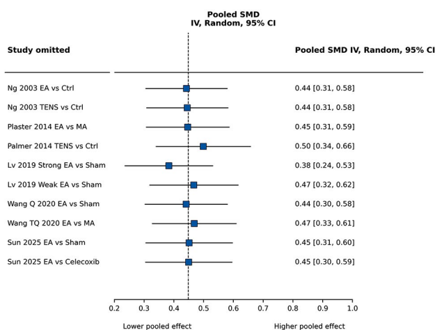
FIGURE 7. Leave-one-out sensitivity analysis of the continuous-outcome model.
