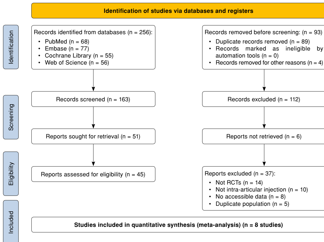
FIGURE 1. PRISMA study flowchart.
