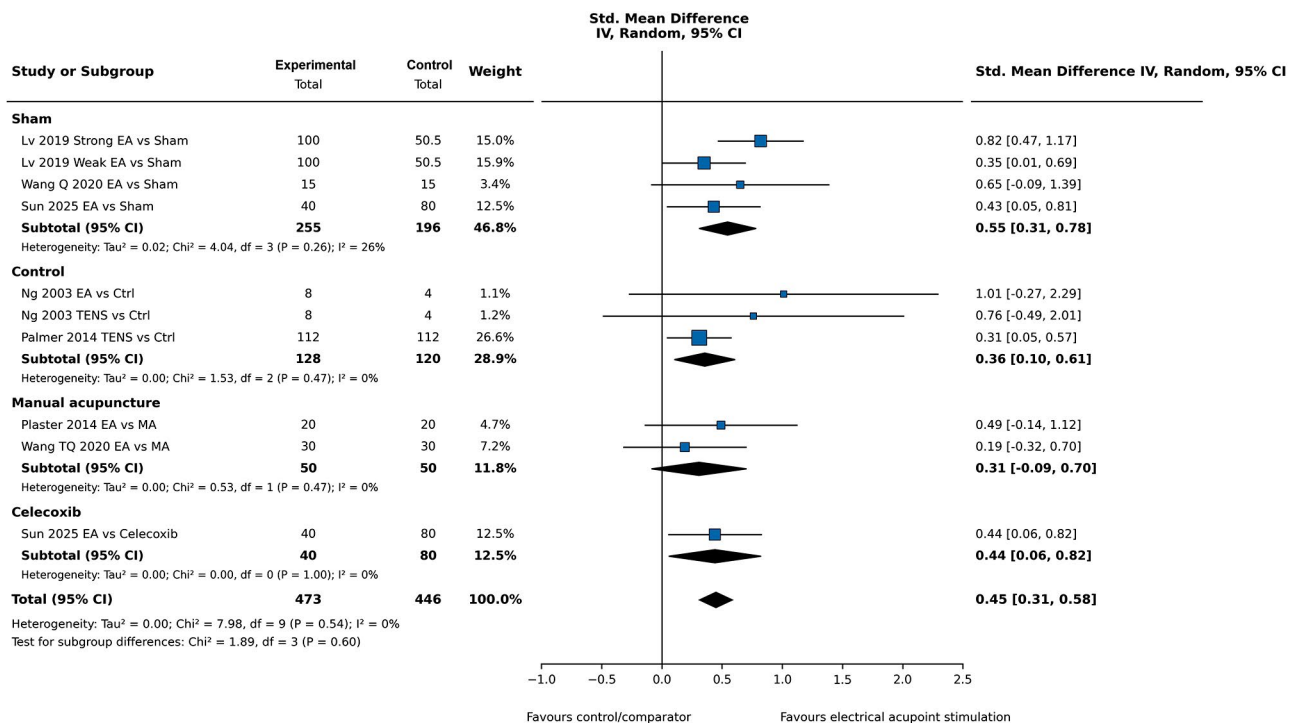
FIGURE 6. Subgroup analysis by comparator type using continuous outcomes only.
