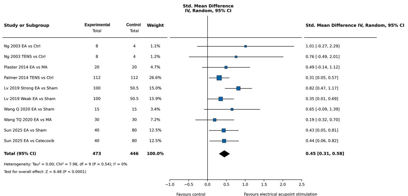
FIGURE 4. Forest plot of the continuous-outcome meta-analysis after multi-arm shared-group correction (random-effects model, Hedges' g).
