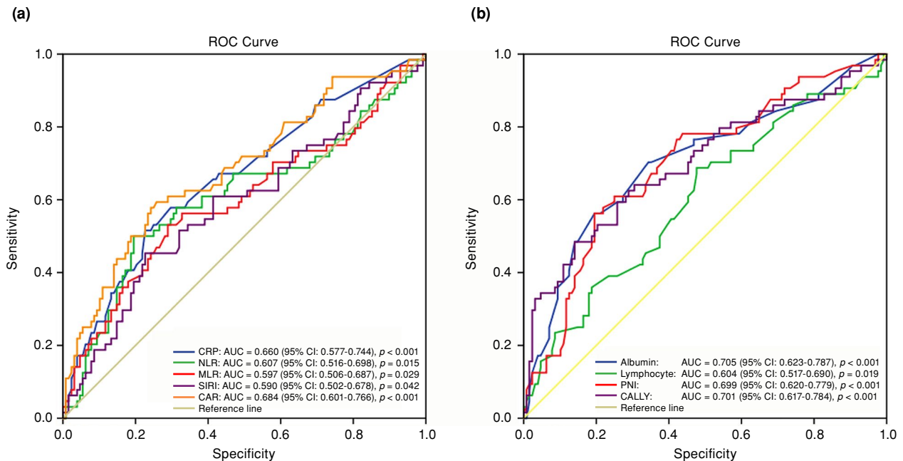
FIGURE 1. ROC curves of inflammatory and nutritional biomarkers for predicting PJI. (a) ROC curves for CRP, NLR, MLR, SIRI, and CAR. Higher values indicate a greater likelihood of PJI. (b) ROC curves for albumin, lymphocyte count, PNI, and CALLY index. Lower values indicate a greater likelihood of PJI. Higher AUC values indicate better discriminatory performance.
